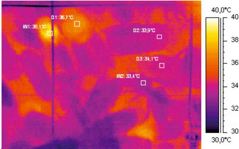
Figure 1. Thermogram of endothermic and ectothermic drones (D) and workers (W) on a comb. Values beside squares indicate the mean thorax temperature of the insects (D1: 36.7 °C, D2: 33.9 °C, D3: 34.1 °C, W1: 38.1 °C, W2: 33.4 °C). Ambient air temperature: ~33.0 °C.
